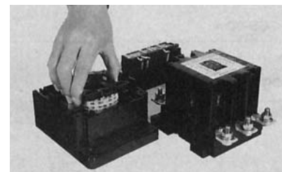
Ⓒ1) Replace to prescribed coil. Ⓒ2) Reassemble in order Ⓑ2)-Ⓑ1)-Ⓐ1) Ⓒ3) Control unit must be suit for replaced coil, and must be replaced with coil at the same time. Ⓒ4) Coil terminals for excepting 100/200V coil are Ⓒ1)-Ⓑ2). Ⓒ5) Secure transparent dustproof covers on both sides.
