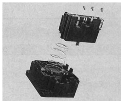
Ⓑ1) After removing Insulating cover, loose 3 screws of coil terminals. Ⓑ2) Remove control unit and return spring.
